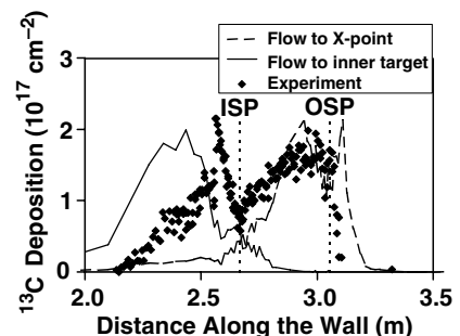
Fig. 3. ELM-dependent deposition hypothesis. Net deposition is the sum of the two results. Inner strike point (ISP) and outer strike point (OSP) are shown.
