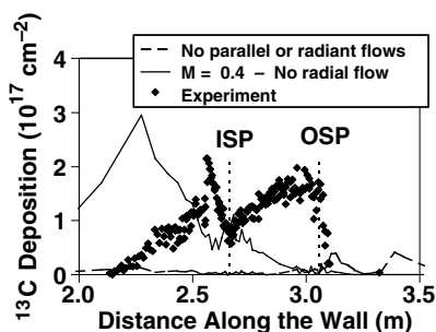
Fig. 5. Flow dependence of deposition. Results shown are for simulations with no parallel flow and no radial flow.
