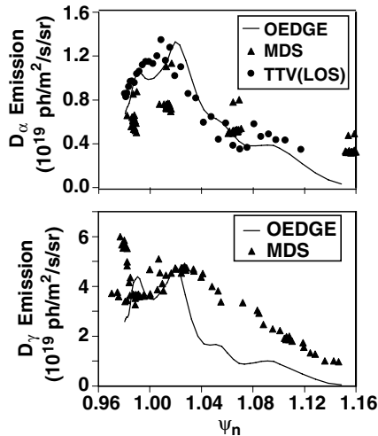
Fig. 2. Comparison of the experimental and modeled D_{\alpha} and D_{\gamma} spectroscopy at inner target. The modeled hydrogen spectroscopy is produced by EIRENE using the OSM plasma solution as input.
