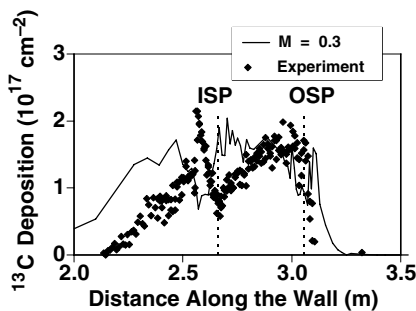
Fig. 4. ELM-independent deposition hypothesis. ^{13}\text{C} is deposited across the inner target and the PFZ using a single set of transport assumptions.
