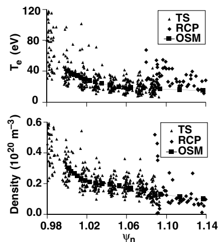
Fig. 1. Comparison of upstream n_e and T_e from Thomson (TS), reciprocating probe (RCP), and the OSM solution for the ^{13}\text{C} H-mode experiment. \Psi_n is the normalized poloidal flux magnetic coordinate.
